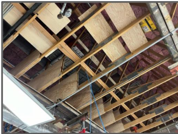
Abia Judd Elementary School Truss Construction
